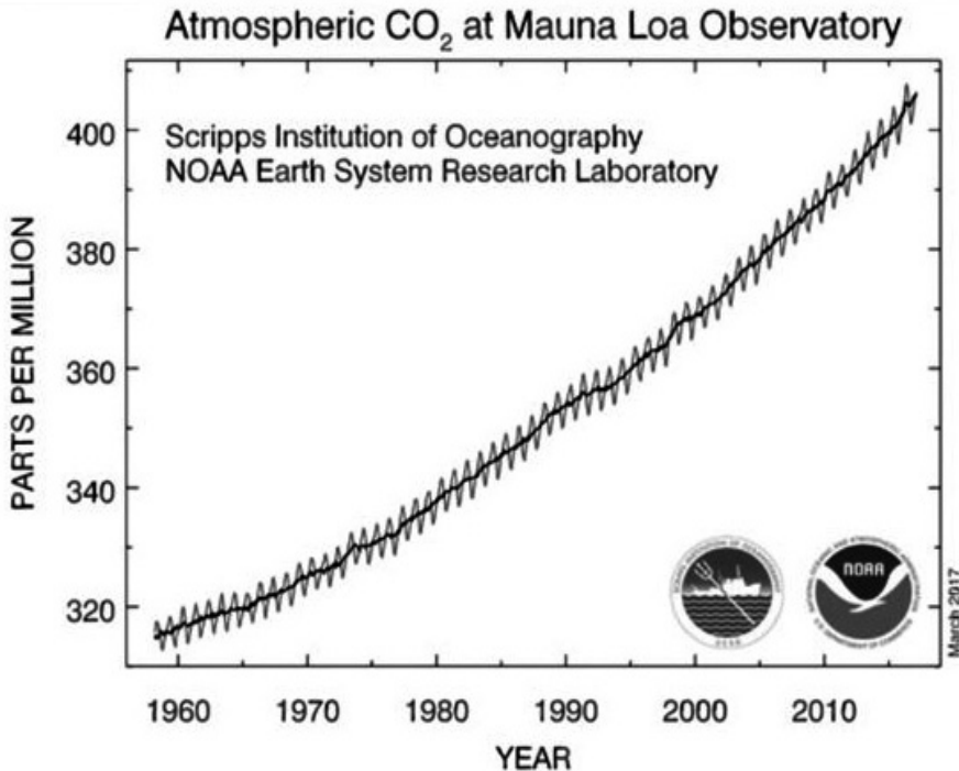
Figure 2 – Trends in atmospheric carbon dioxide. Source: NOAA Earth System Research Laboratory ( https://www.esrl.noaa.gov/ )
